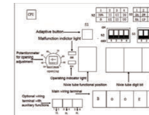
Fig.8: Control Panel - Intelligent Proportional Control 1800/3000/5000N (24VAC)
