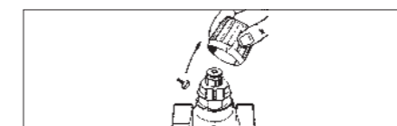
Fig.2 Unscrew the locking screw and remove the handwheel, taking care not to turn the control stem, and taking note of the corresponding setpoint for subsequent refitting.
