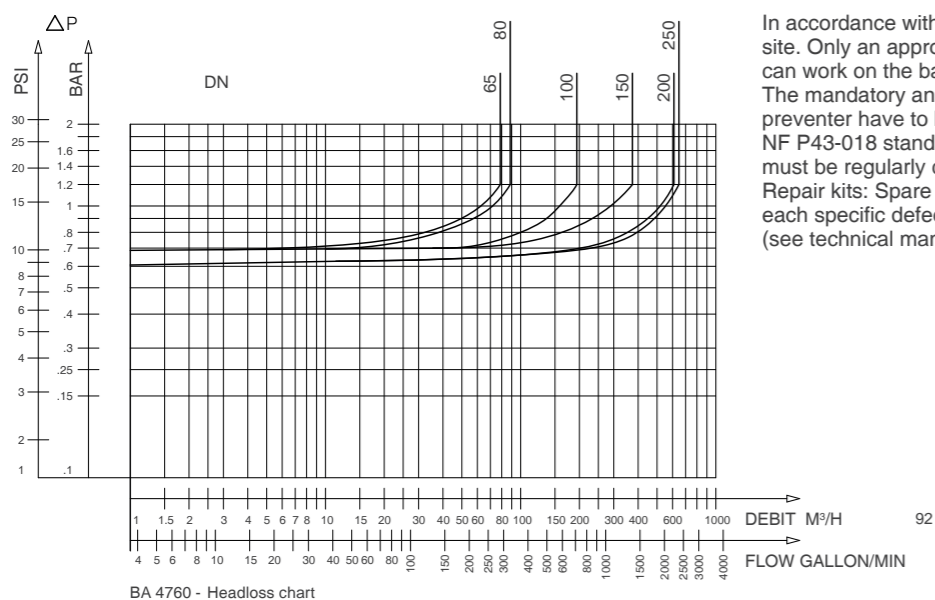
BA 4760 - Headloss chart
