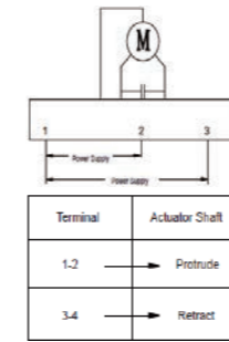
Fig.4: Floating Point Control Wiring 500/1000N
