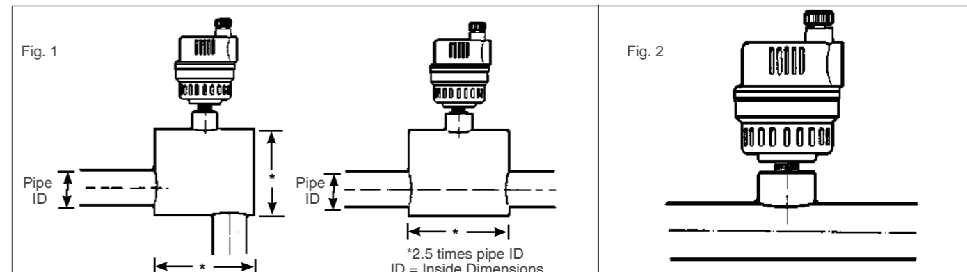
Figure 1 shows the installation of the FV-4M1 for the venting of air while the fluid is circulating in the system. The figure shows the required increase in pipe size in order to obtain proper separation of air from water. Watts Series AS Air Scoop which is designed for efficient separation of air from water in hydronic heating systems can also be installed. See Watts literature S-AS.
