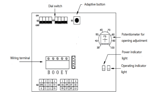
Fig.6: Control Panel - Intelligent Proportional Control 500/1000N (24VAC)
