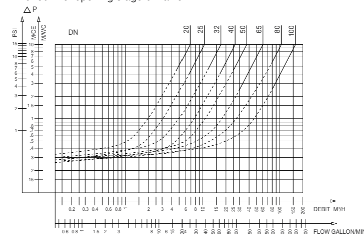
60S - Headloss chart
