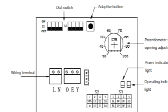
Fig.7: Control Panel - Intelligent Proportional Control 500/1000N (220VAC)
