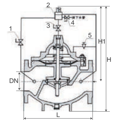
1.Small Ball Valve 2.Pilot Valve 3.Small Ball Valve 4.Small Ball Valve 5.Needle Valve
