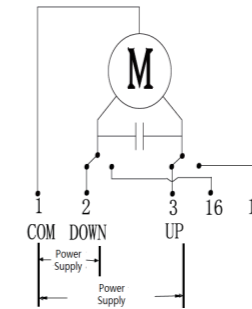
Fig.5: Floating Point Control Wiring 1800/3000/5000N
