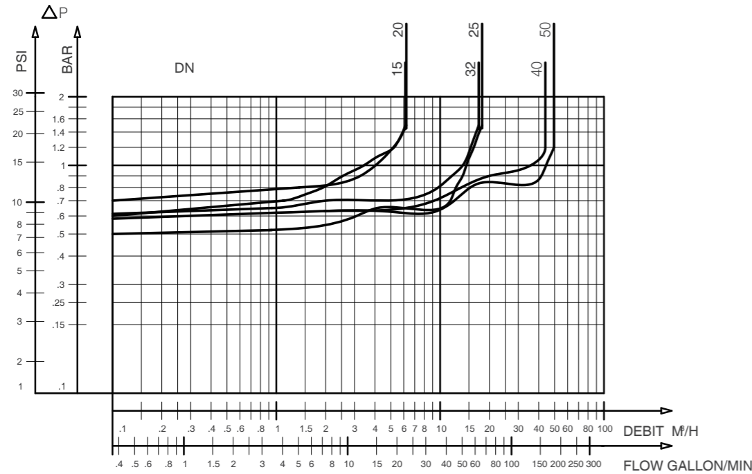
BA BM-Headloss chart
