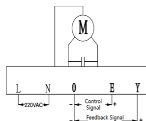
Fig.2: Intelligent Proportional Control Wiring 500/1000/1800/3000/5000N (220VAC)
