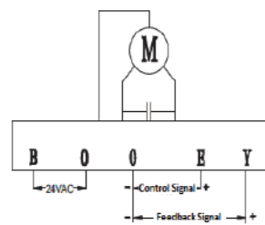
Fig.1: Intelligent Proportional Control Wiring 500/1000/1800/3000/5000N (24VAC)
