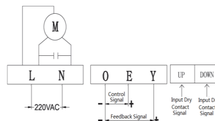
Fig.3: Intelligent Proportional Control Wiring 16000N (220VAC)
