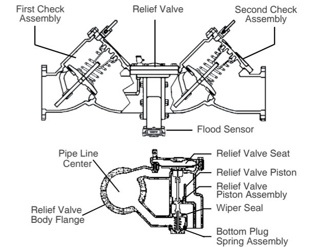
Series LF909-FS Technology integrated for flood detection upon activation with Sensor Connection Kit
