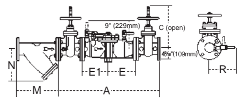
Strainer Dimension
