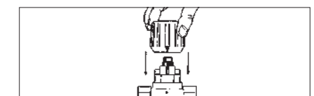
Fig.3 Refit the handwheel so that the V-shaped reference mark lines up with the mark on the valve body. In this position, the handwheel is locked.
