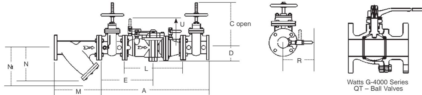
Dimensions – Weight
