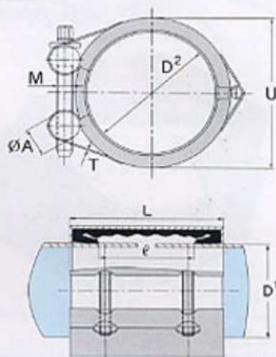
MODEL 6 : RCH-L (REPAIR CLAMP HINGE LONG)
