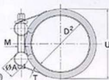
MODEL 3: MF-RS (MULTI-FLEX ROUND STANDARD)
